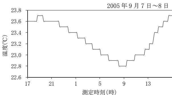
Fig.2-11 堤体表面温度(天端)の日変化(六道池) Daily fluctuations of the dam body surface temperature
