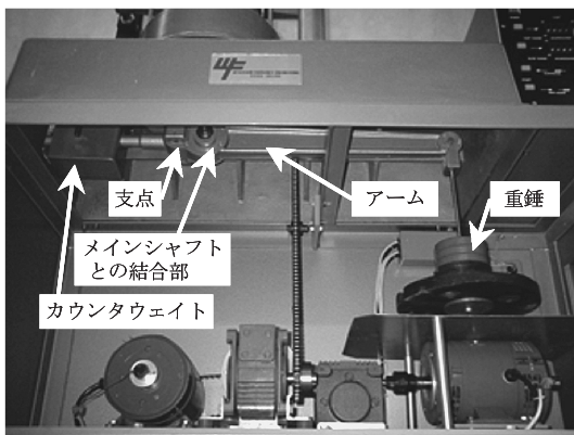
Fig.6 基本枠内側 Inside the base frame
