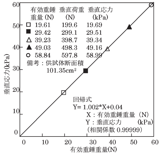
Fig.14 有効重錘重量と垂直応力の関係 Relationship between dead load and normal stress
