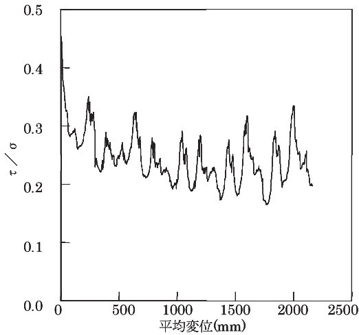
Fig.19 \tau/\sigma -変位関係 (プレカット試料, 先行載荷) \tau/\sigma -displacement relationships (pre-cut sample, preliminary loading)
