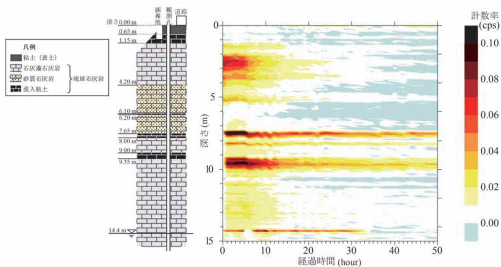
Fig.4 中性子水分検層の結果および涵養施設の断面図 Result of neutron moisture logging and section view of the test facility
