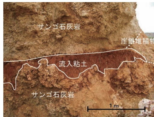
Fig.2 露頭で観察される流入粘土 Influent mud observed at outcrop
