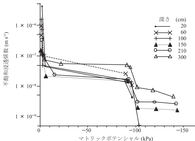
Fig.6 チョーク上部層における不飽和透水係数とマトリックポテンシャルの関係 (Wellings, 1984a) Relationship between unsaturated permeability and matric potential for the Upper Chalk
