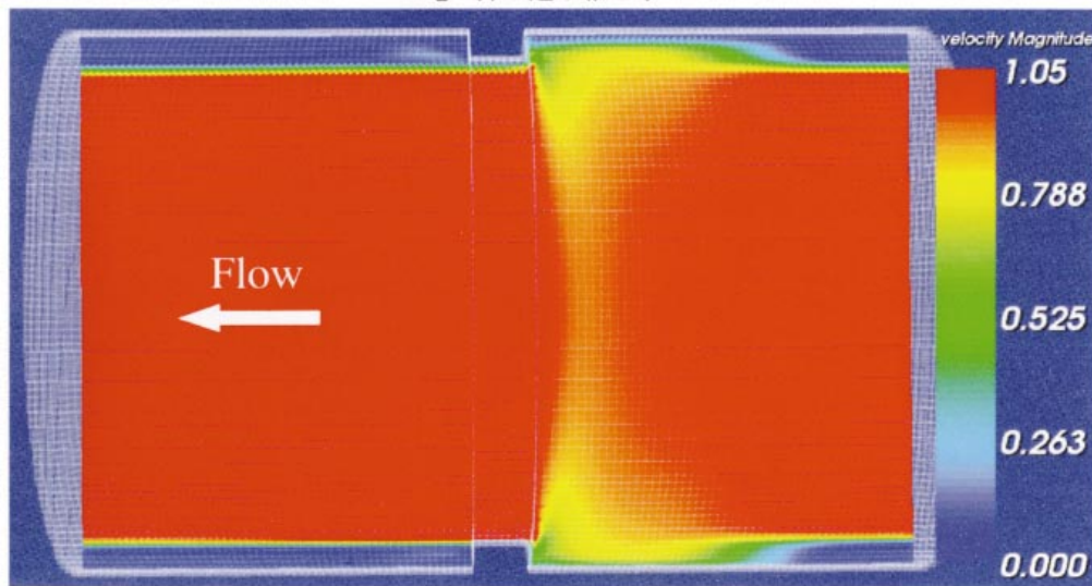
Fig.12 管内の流速分布 Flow distribution in pipe
