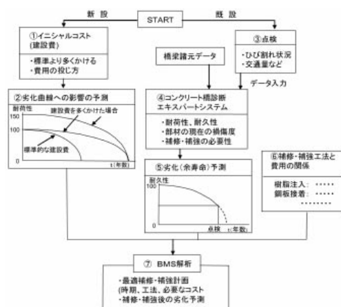
Fig.7 Bridge Management System (BMS)の概要 (宮本ら, 1997)
