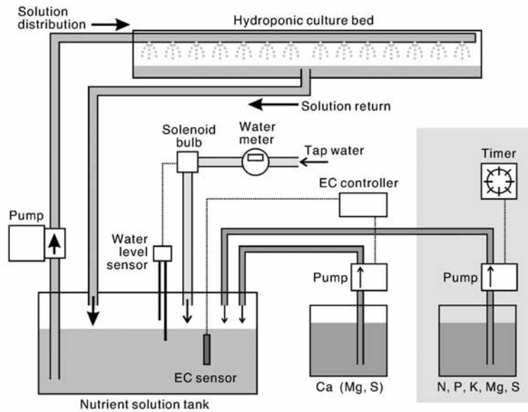
Fig. 1 System of tomato hydroponic cultivation to ensure that no N・P・K manure elements remain in the culture solution.
