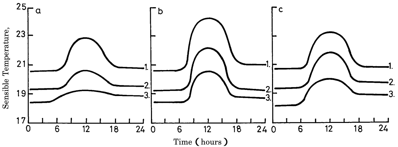
Fig. 9 Diurnal variation in sensible temperature at 1.5 m for (a) paddy canopy, (b) field (upland) crop, and (c) grassland in July 1996.
