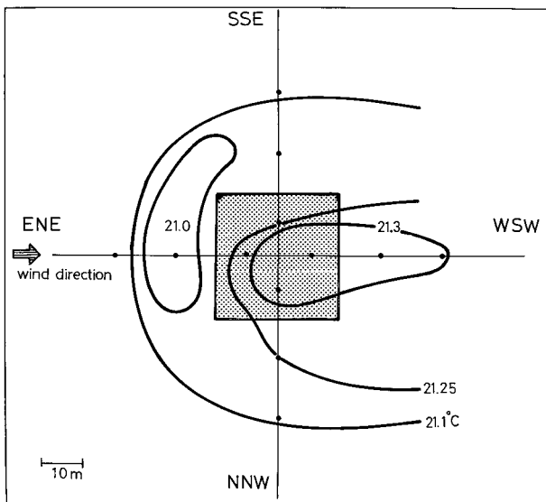
Fig. 5 Spatial distribution of air temperature at z=1 m in the observation field during 3 months in 1996. The prevailing wind direction was ENE.
