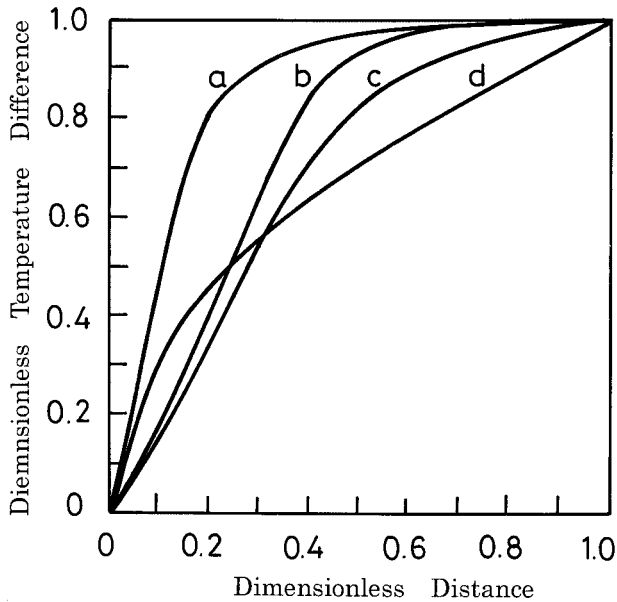
Fig. 4 Dependence of temperature changes ( T/T_{max} ) dimensionless by maximum temperature change ( T_{max} ) on dimensionless fetch ( x/X ) under 4 conditions. T_{max} denotes the temperature changes ( T_{max} ) at maximum fetch ( X ) of experimental field.
