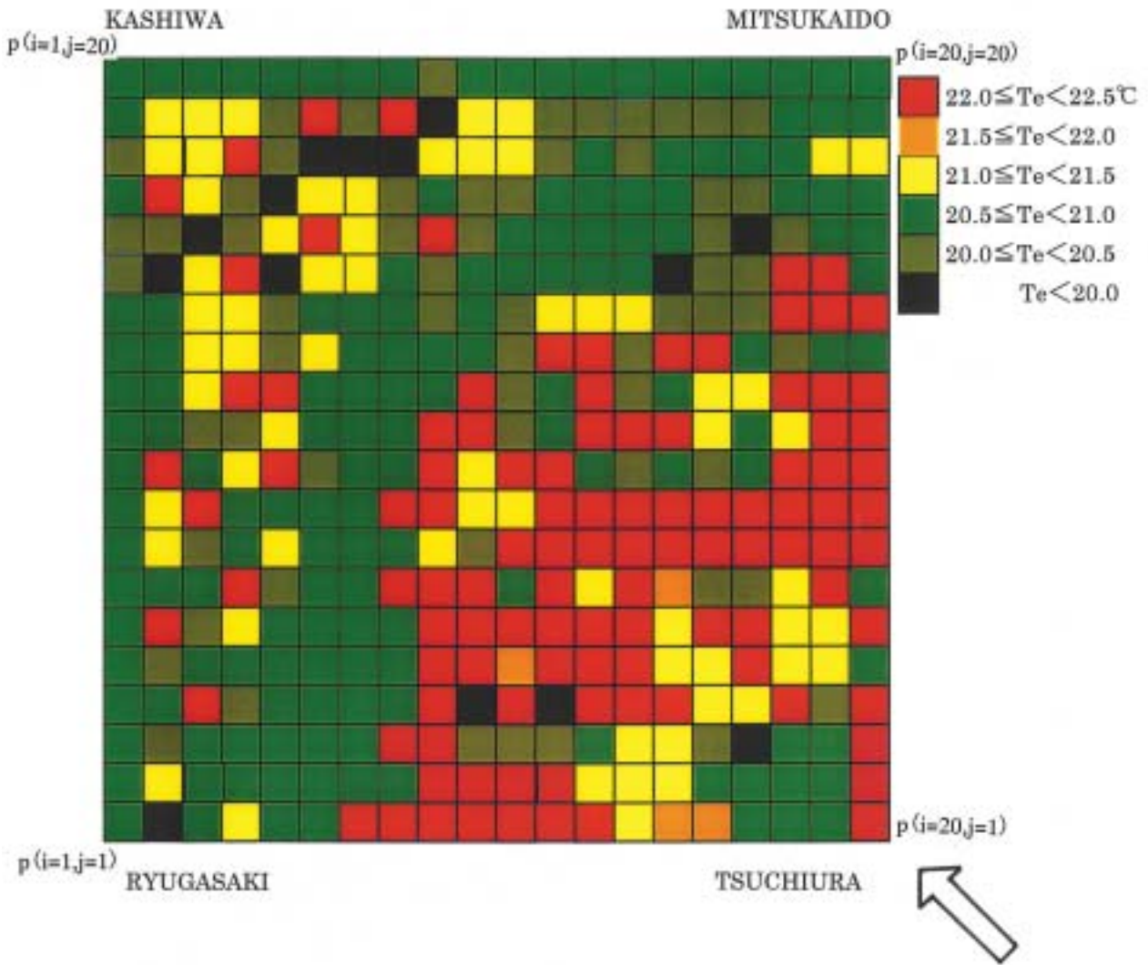
Fig. 8 Spatial distribution of monthly mean sensible temperature at 1.5m in experimental fields with different land-use plots at 12:00 JST in July 1996.
