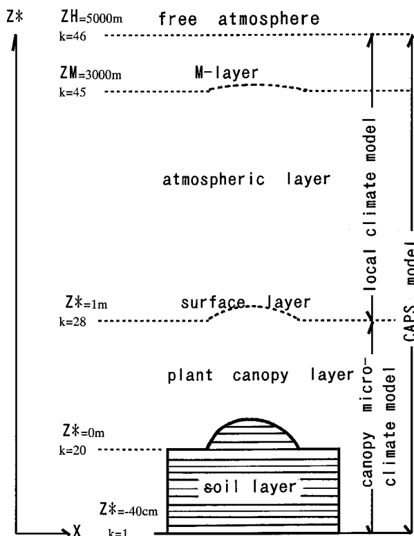
Fig. 1 Internal configuration of CAPSM used in simulation experiments.
