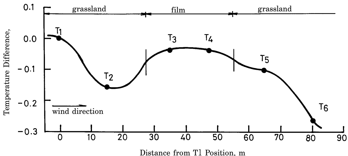
Fig. 6 Change in air temperature at z=1 m with prevailing wind direction in grassland during 3 months in 1996. Temperature differences indicate differences in air temperature between upwind edge (T1) and at each point (T2-T6).
