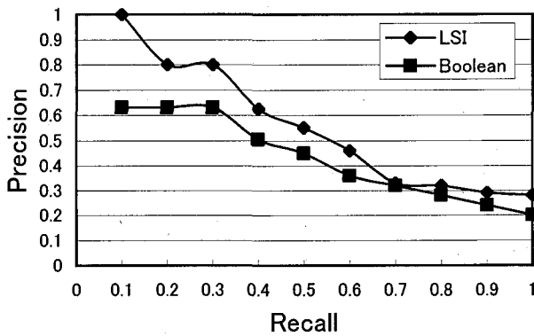
Fig. 4 . An evaluation result of the retrieval method.
