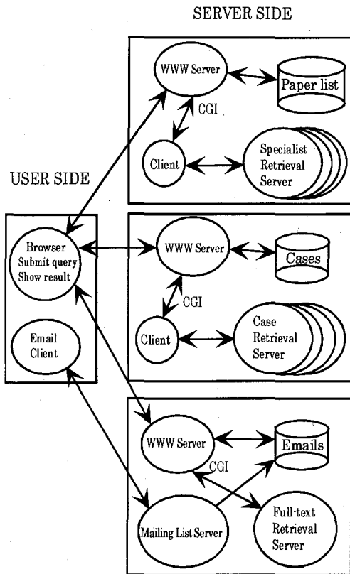
Fig. 1 . Schematic diagram of Agriculture Case Base.
