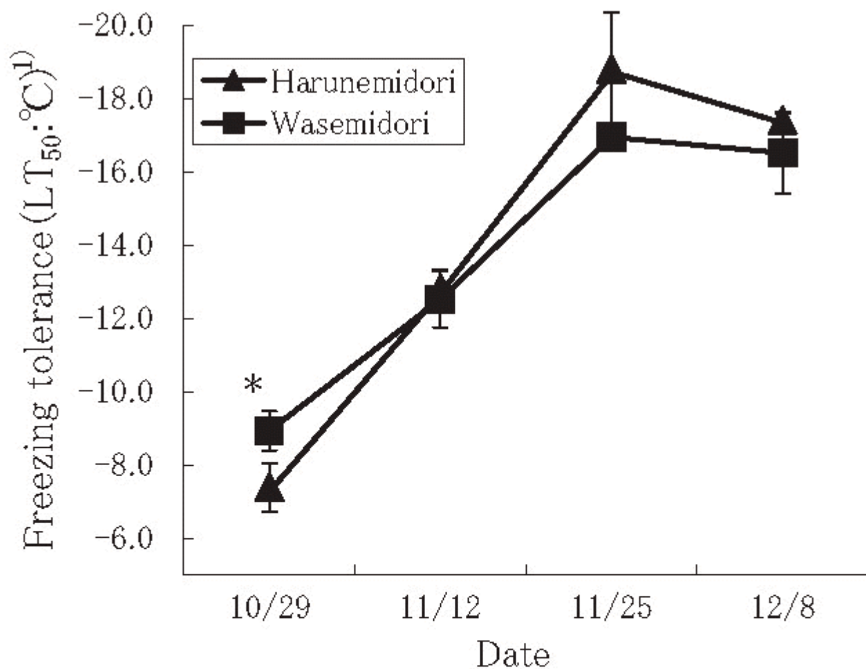
Figure 2. Changes in freezing tolerance in autumn (Sapporo, 2003).
