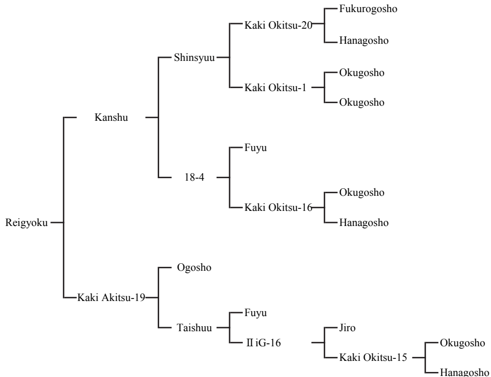
Fig. 1 Pedigree of ‘Reigyoku’
